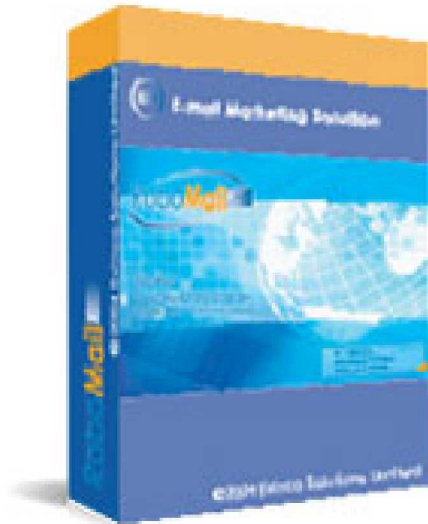
RoboMail Software
