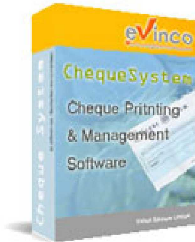
ChequeSystem Software
